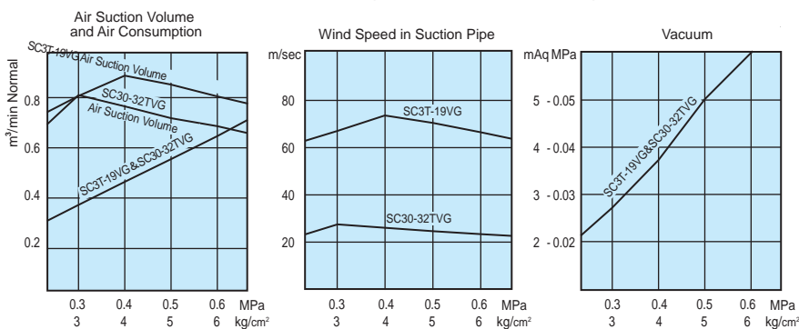
■ Performance Chart( SC30-32TVG,SC3T-19VG )
