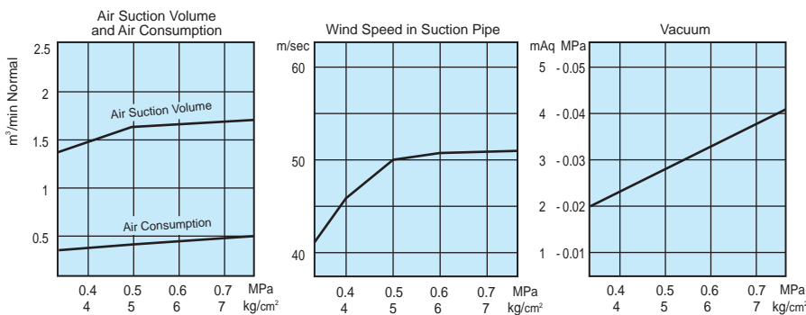
■ Performance Chart ( SC30-32S, SC20-32, SC20-32P )
