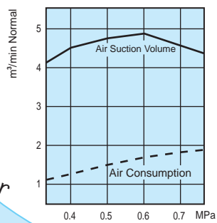
Air Suction Volume and Air Consumption
