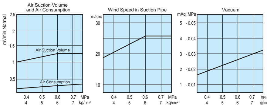
■ Performance Chart ( MP-38WACF12 )
