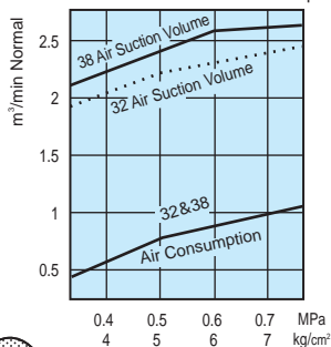
Air Suction Volume and Air Consumption
